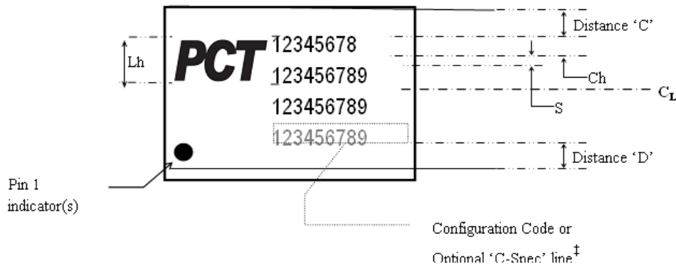
Drawing 11P: 8-SOIC / 150 mil Top Side Mark
