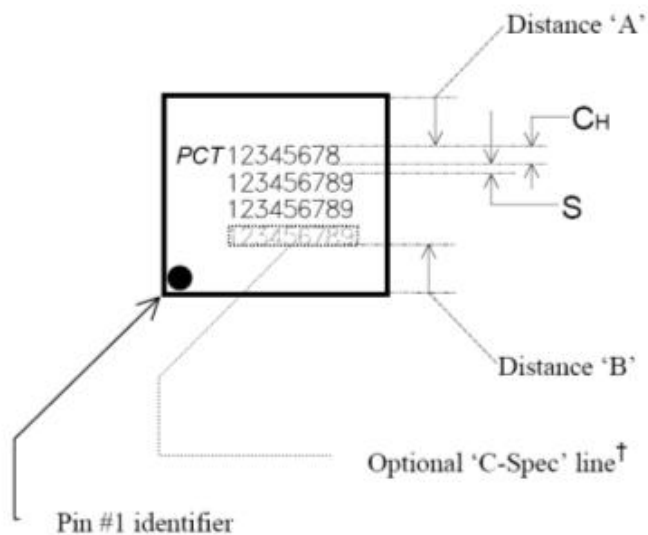
Drawing 12P4: 8-WSON / 5 x 6 mm Top Side Mark (4 line version)
