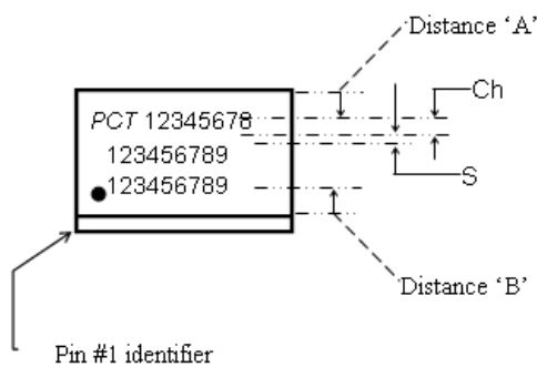
Drawing 11P4a: 8-SOIC / 208 mil Top Side Mark
